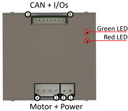
Figure 7: TMCM-1278 connectors
